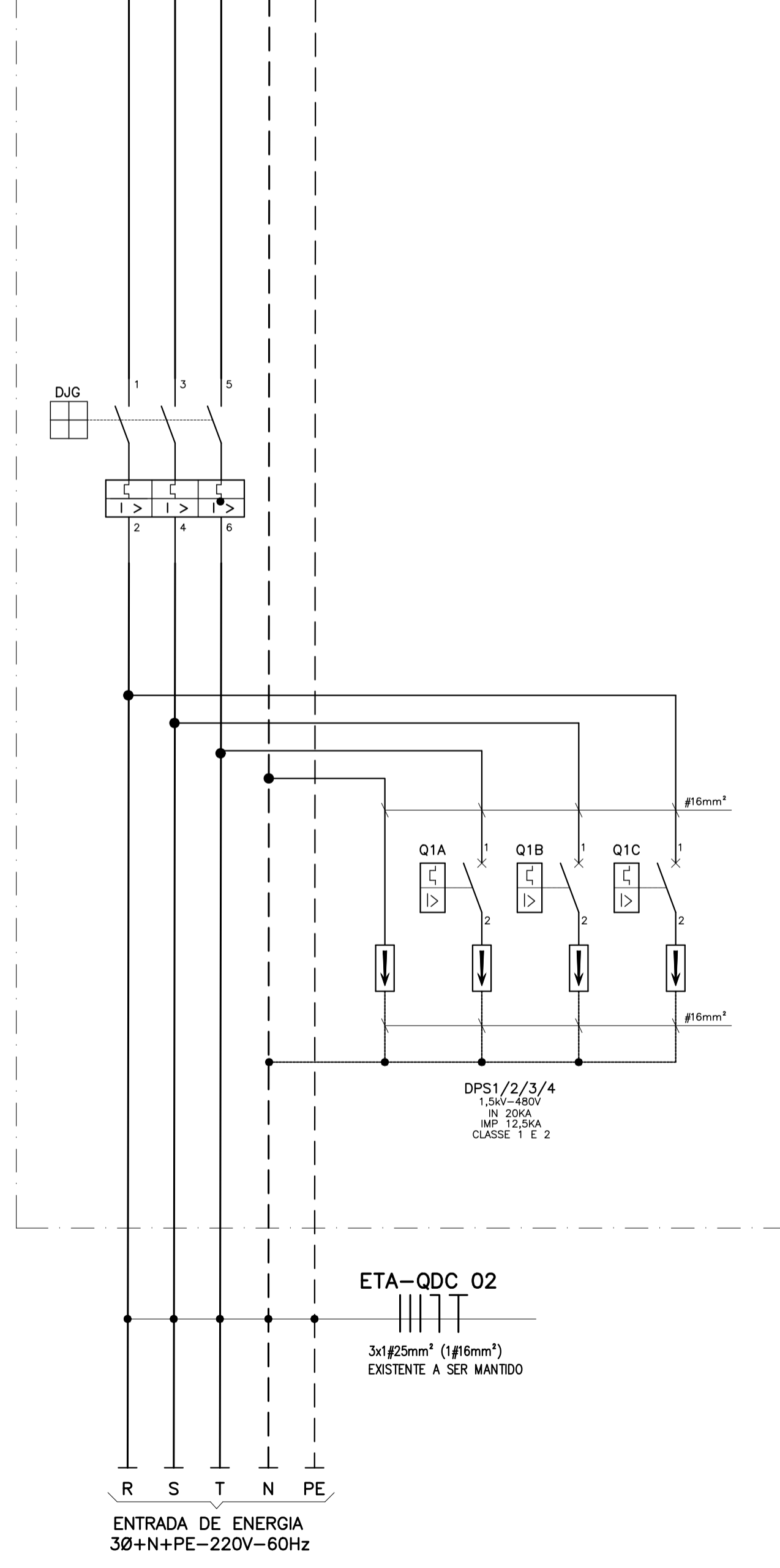
1 DIAGRAMA TRIFILAR
